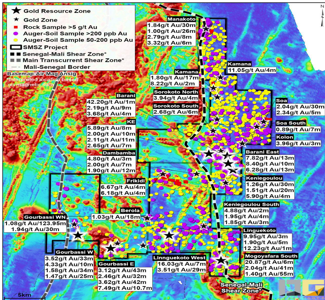
Figure 4. Plan Map Mineral Deposits and Zones, significant drill hole intercepts*, soil geochem summary on color-contoured analytical signal; magnetic data
